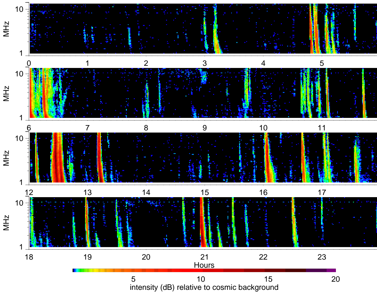
Wind Waves RAD2 receiver: 2004/10/25
