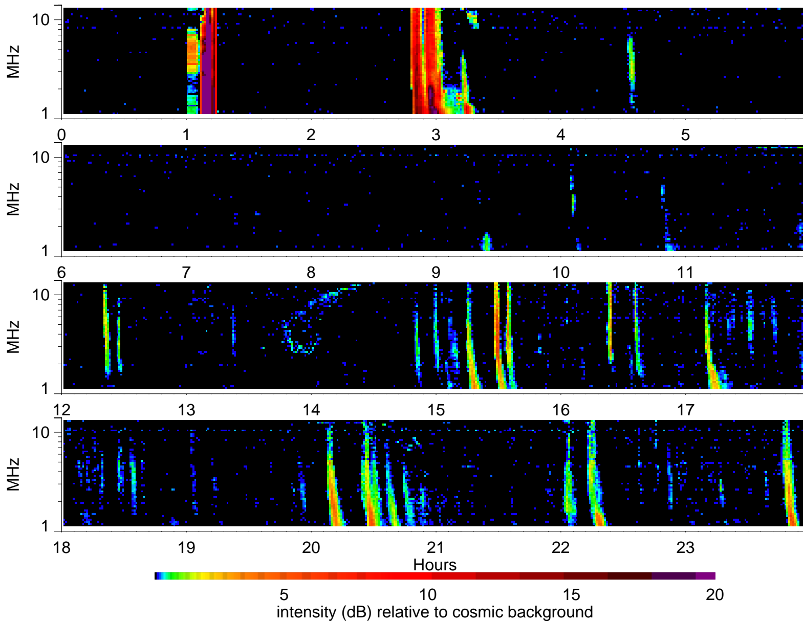
Wind Waves RAD2 receiver: 2004/10/24
