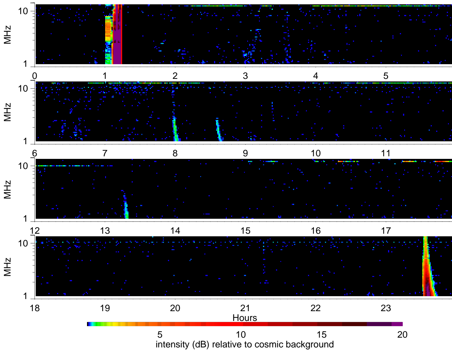
Wind Waves RAD2 receiver: 2004/10/18
