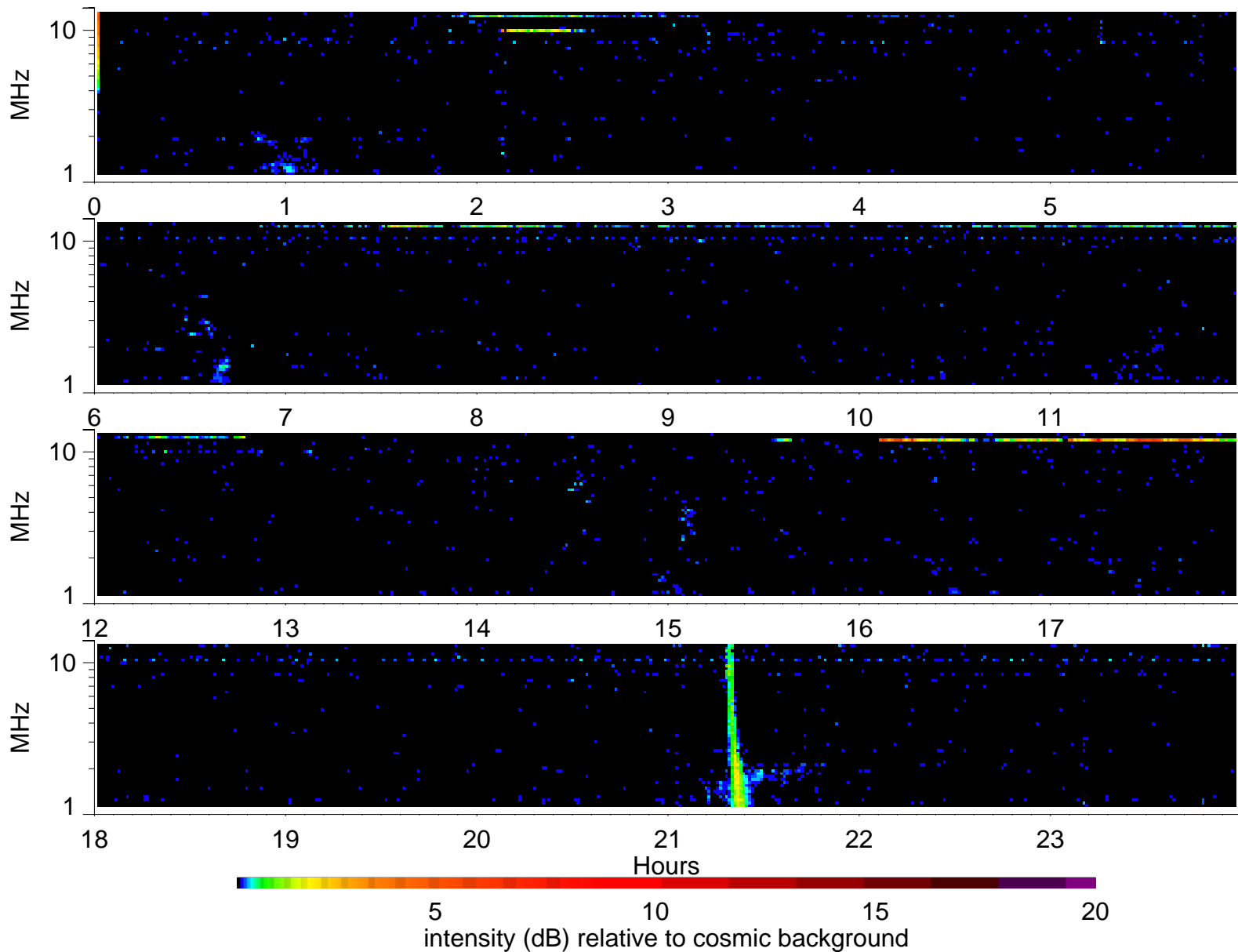
Wind Waves RAD2 receiver: 2004/10/17
