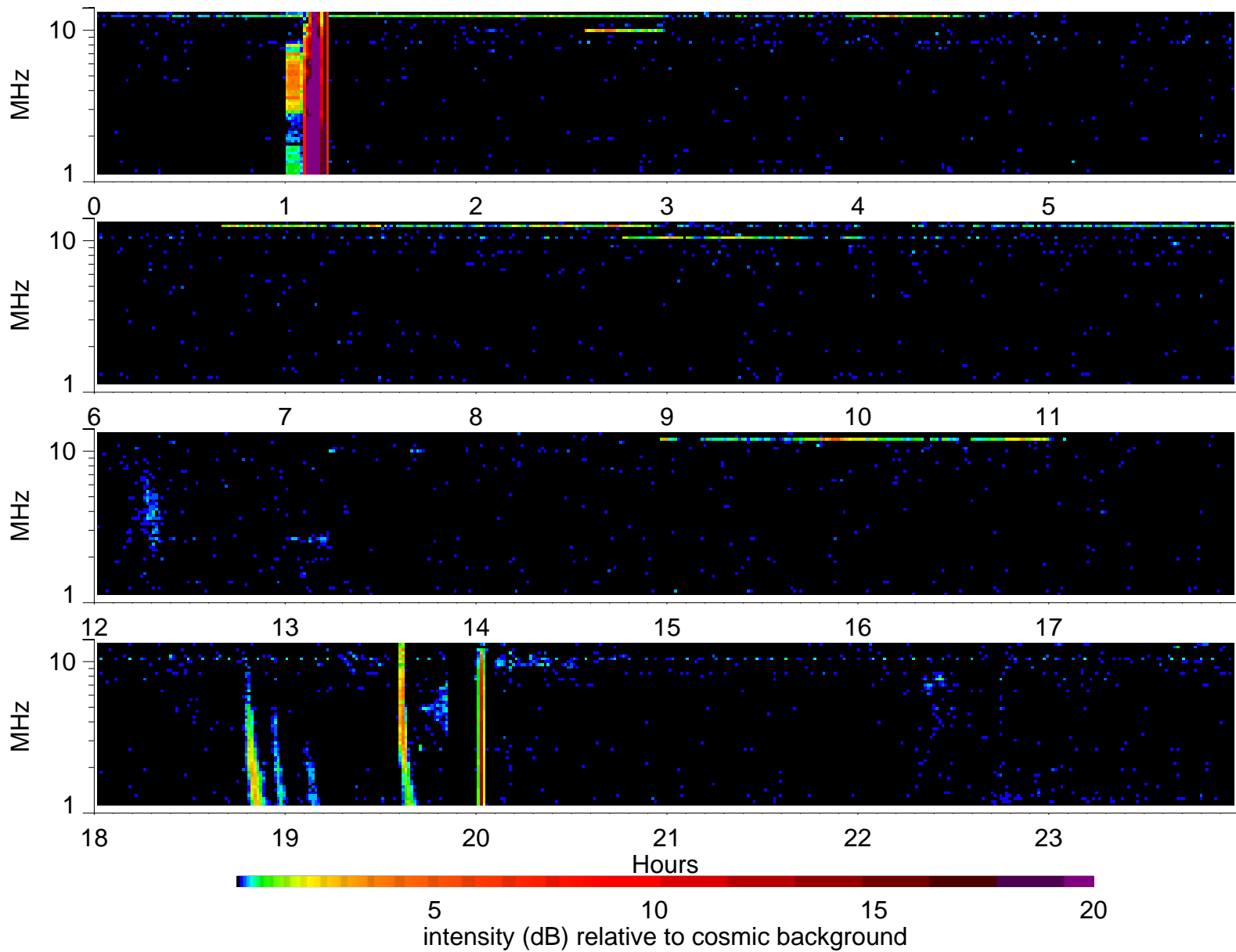
Wind Waves RAD2 receiver: 2004/10/6
