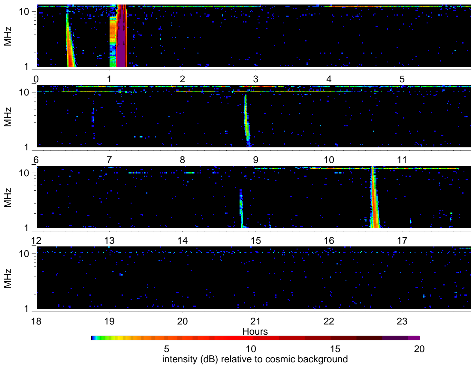
Wind Waves RAD2 receiver: 2004/10/4
