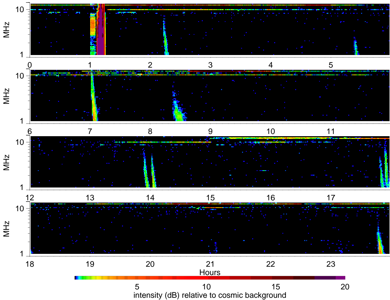
Wind Waves RAD2 receiver: 2004/9/22
