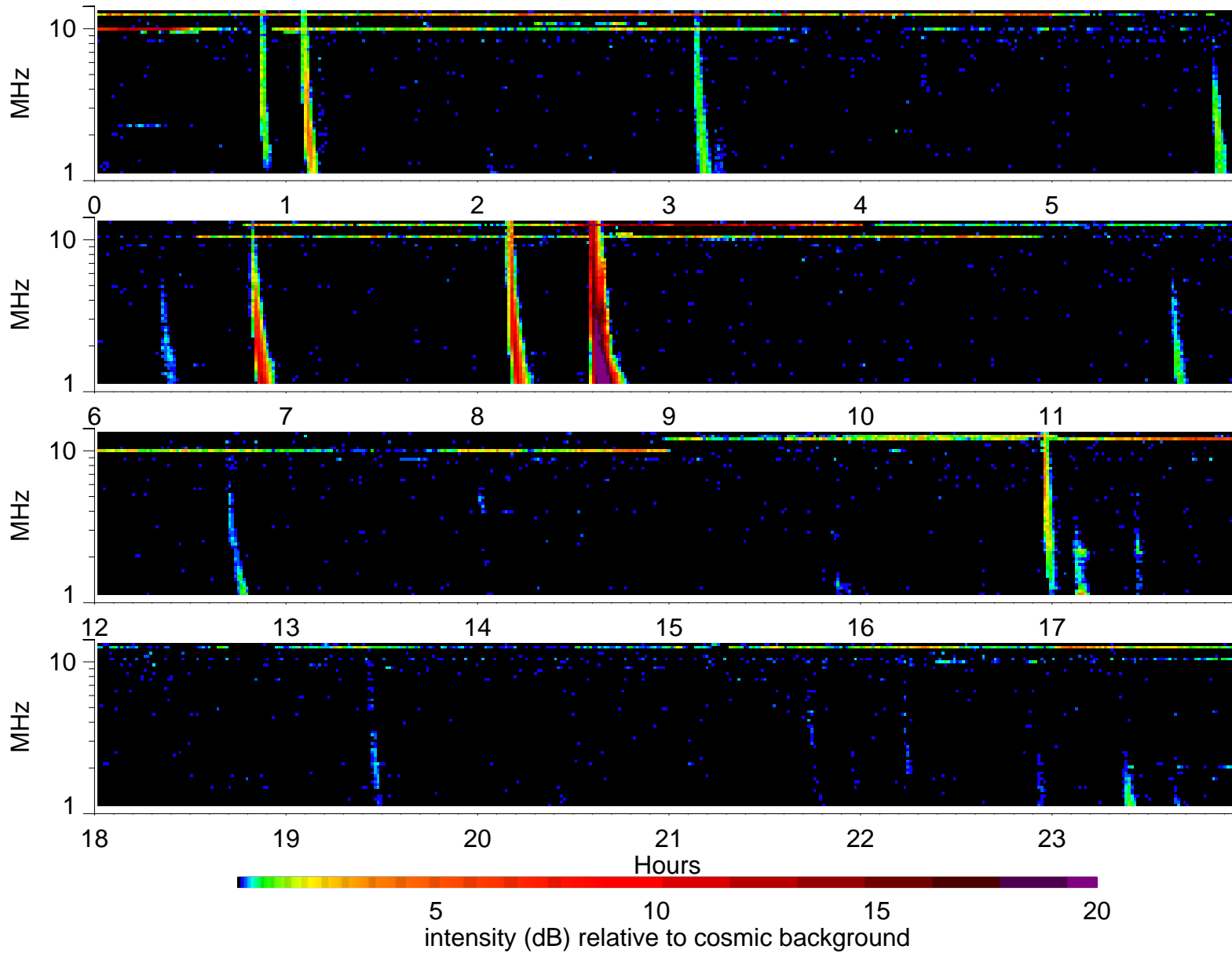
Wind Waves RAD2 receiver: 2004/9/21
