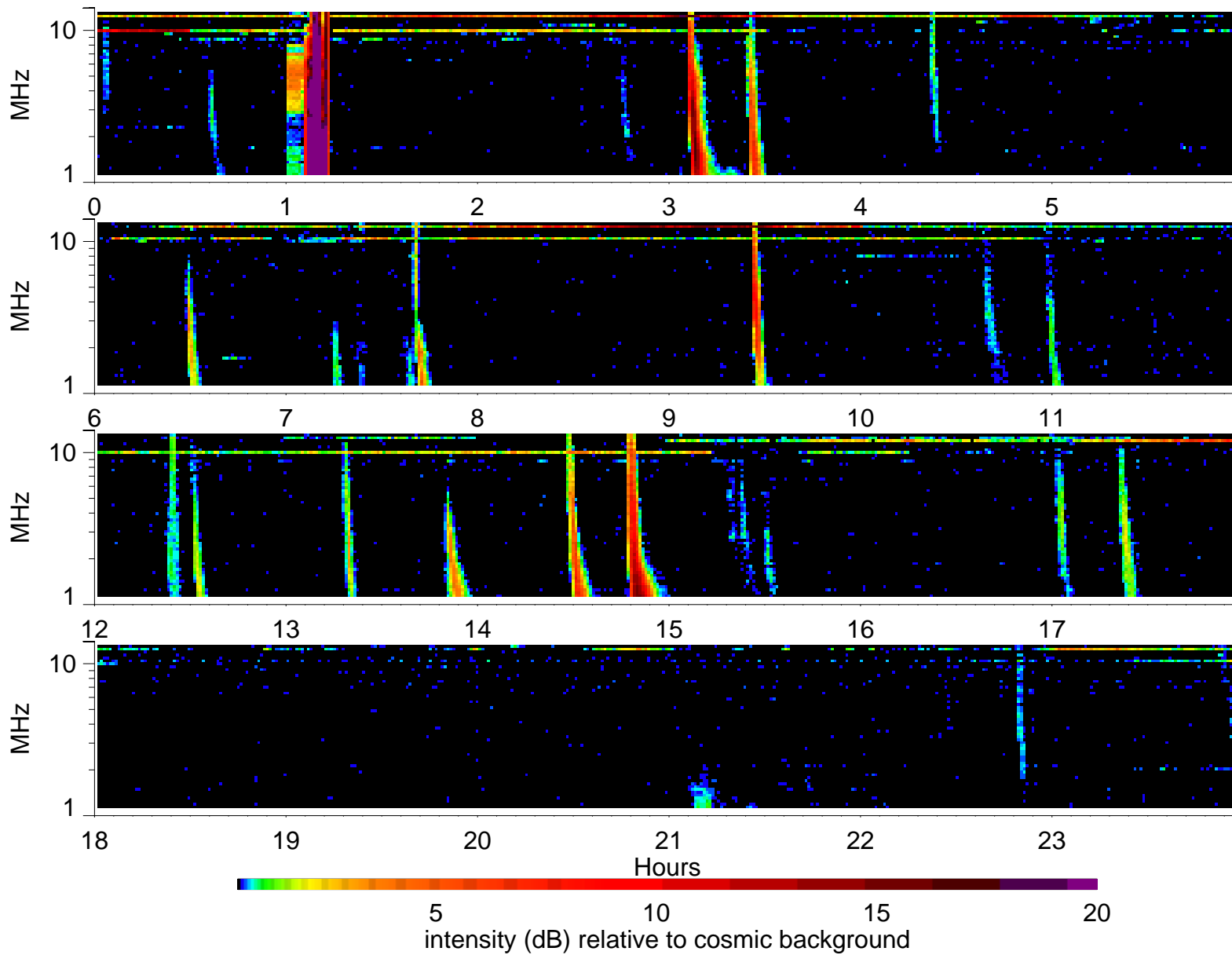
Wind Waves RAD2 receiver: 2004/9/20
