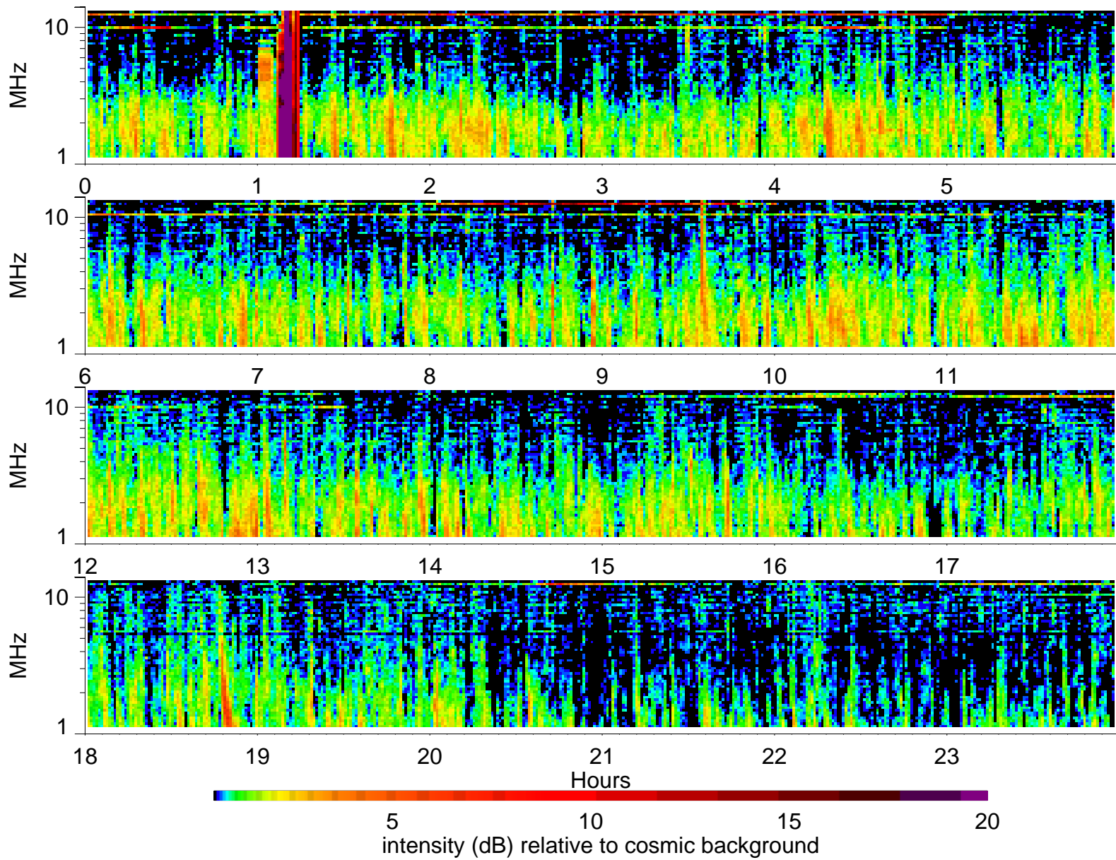
Wind Waves RAD2 receiver: 2004/9/8
