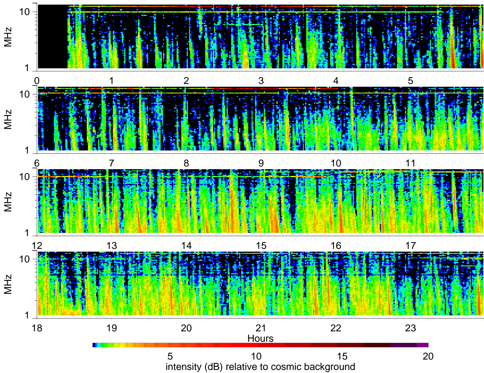
Wind Waves RAD2 receiver: 2004/9/5
