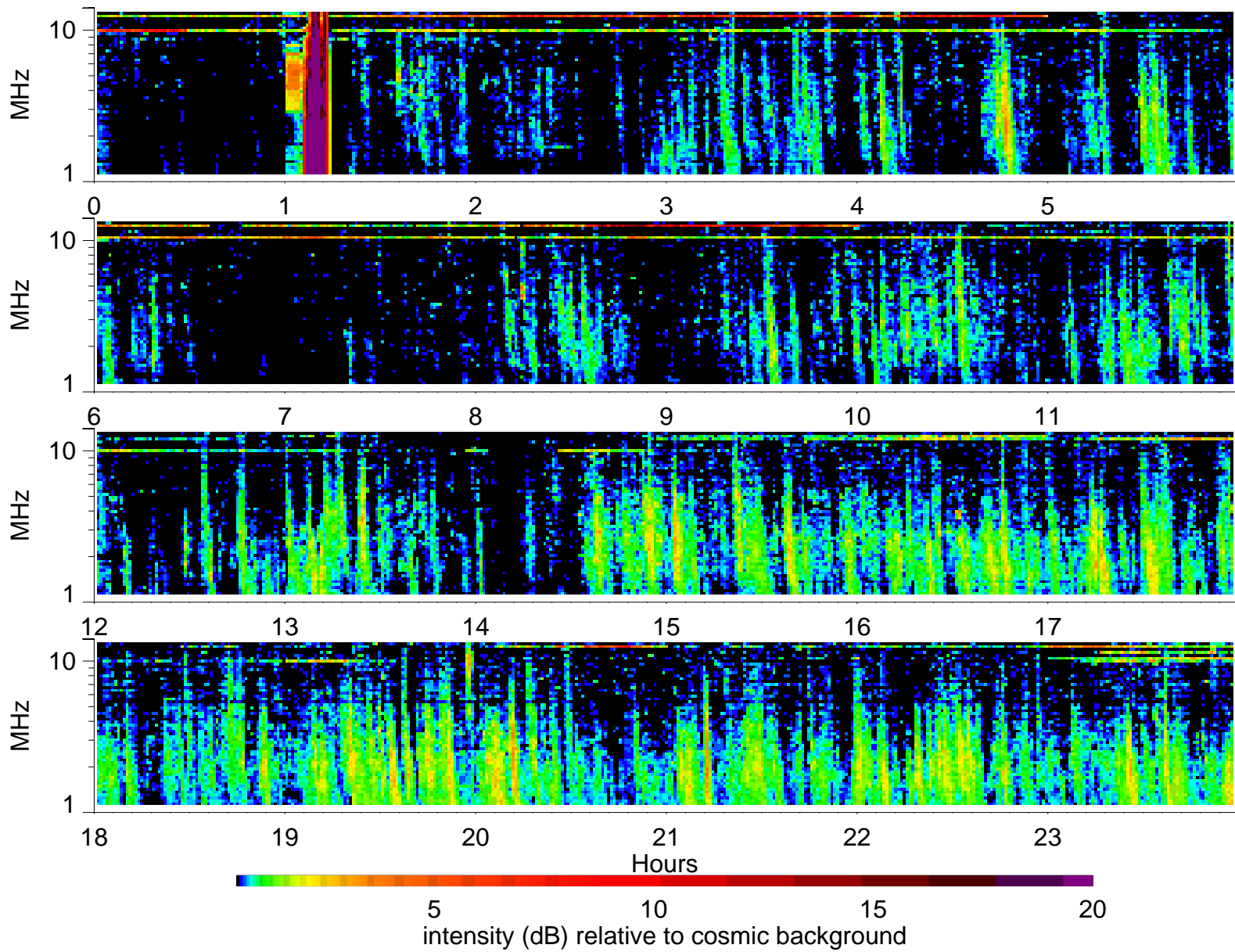
Wind Waves RAD2 receiver: 2004/9/4
