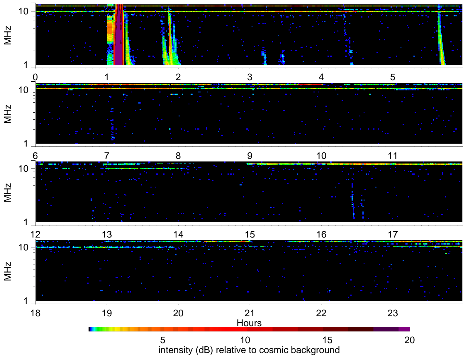
Wind Waves RAD2 receiver: 2004/8/27
