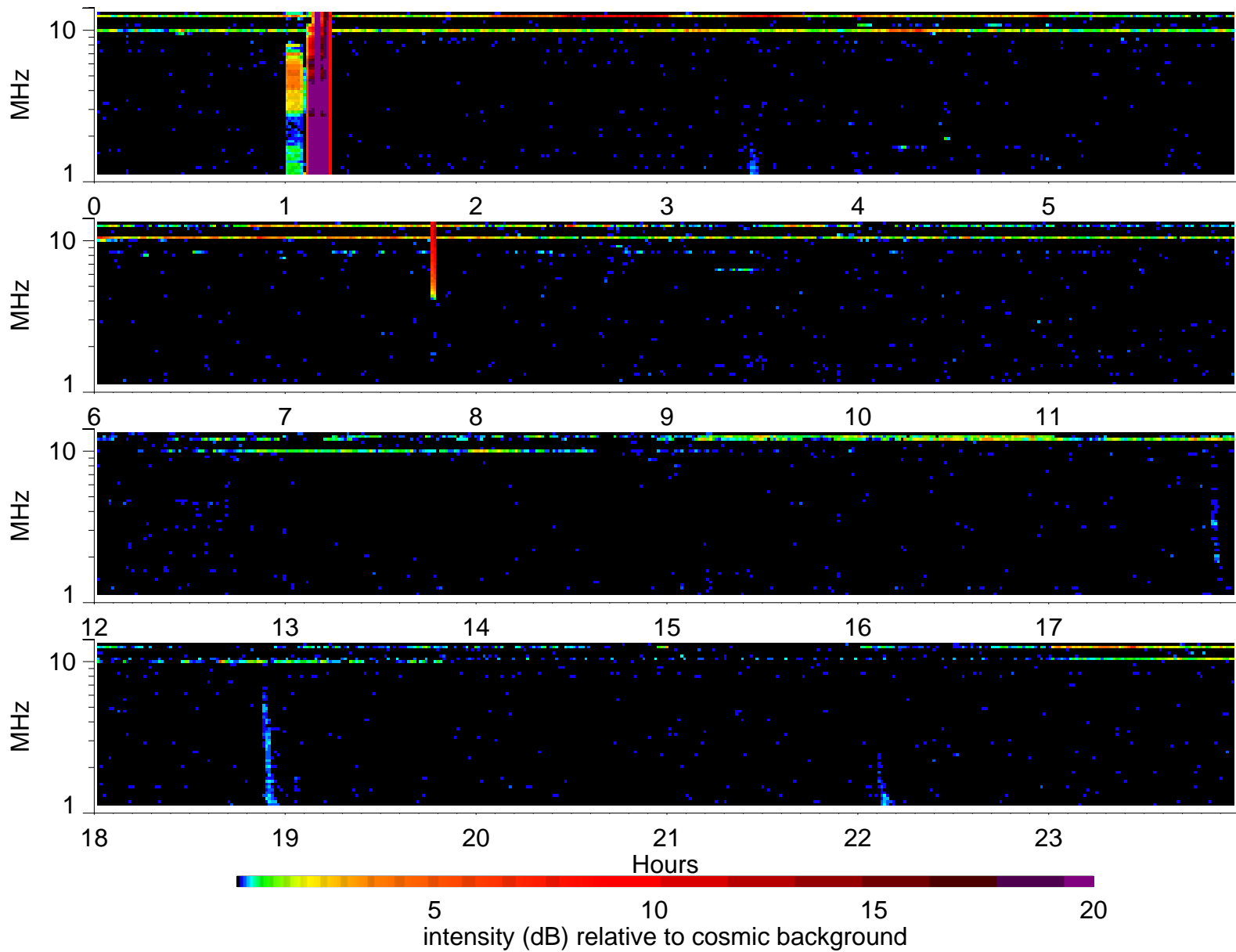
Wind Waves RAD2 receiver: 2004/8/25
