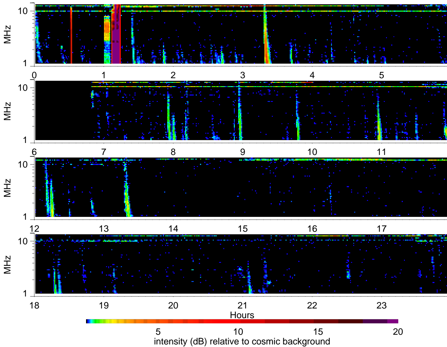
Wind Waves RAD2 receiver: 2004/8/17
