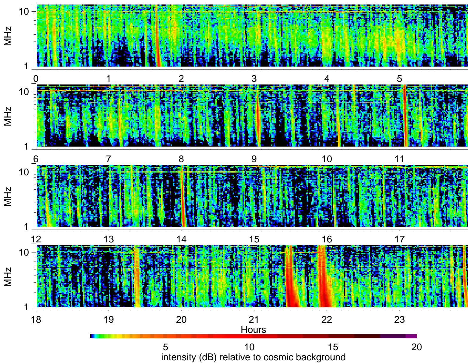
Wind Waves RAD2 receiver: 2004/8/10
