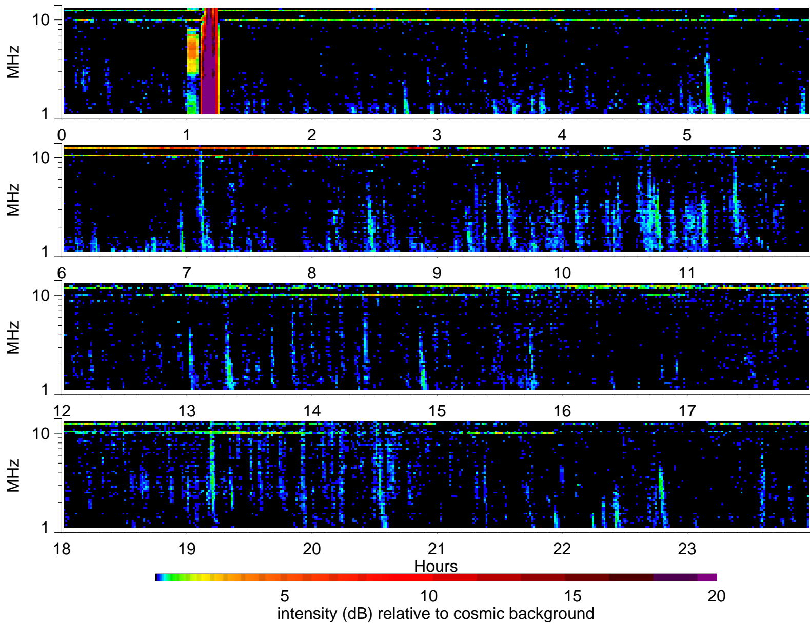
Wind Waves RAD2 receiver: 2004/8/7
