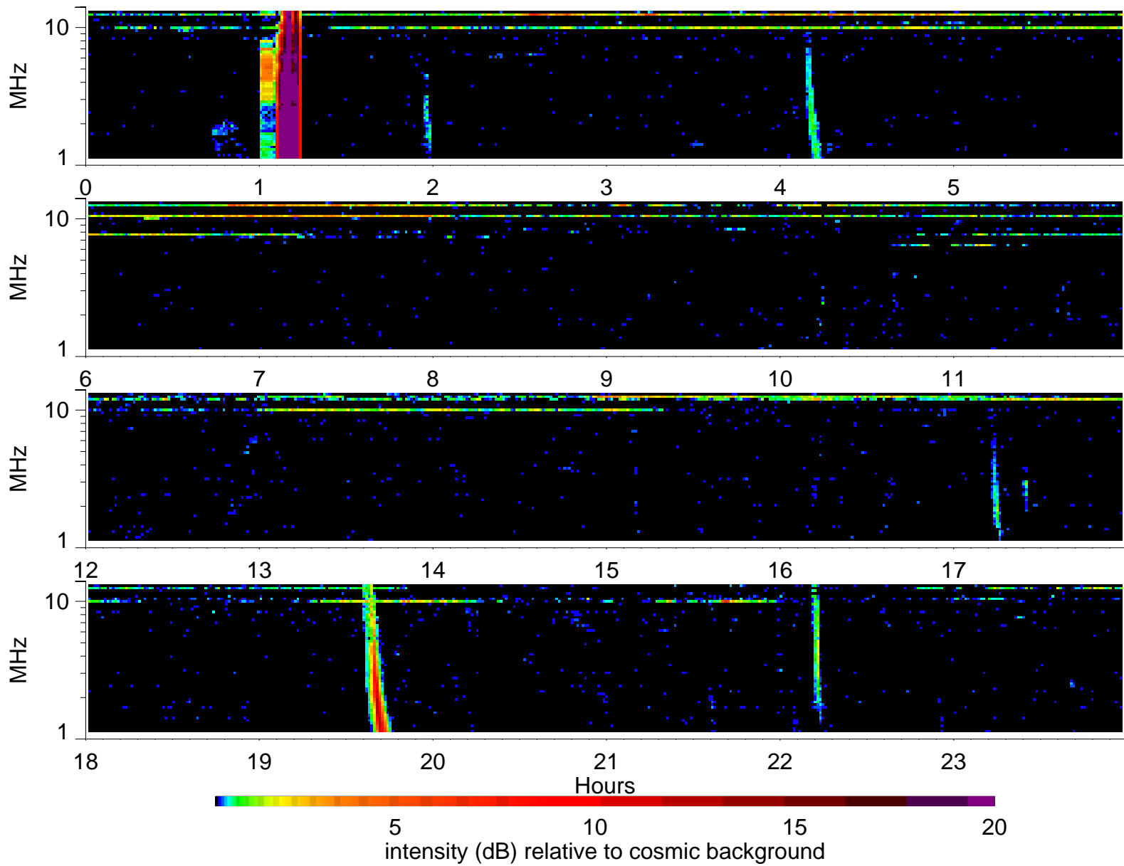
Wind Waves RAD2 receiver: 2004/8/3
