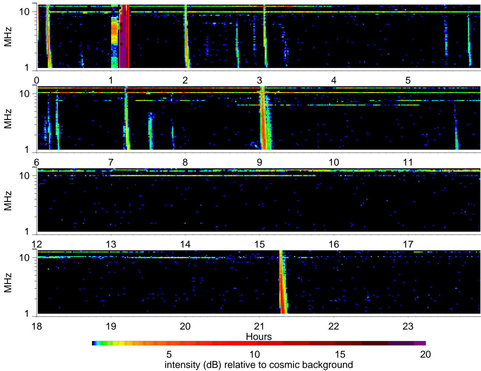
Wind Waves RAD2 receiver: 2004/8/1
