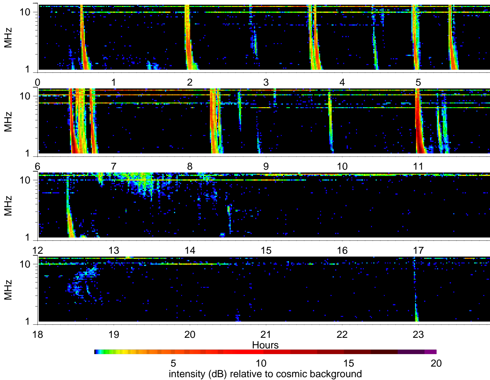
Wind Waves RAD2 receiver: 2004/7/29
