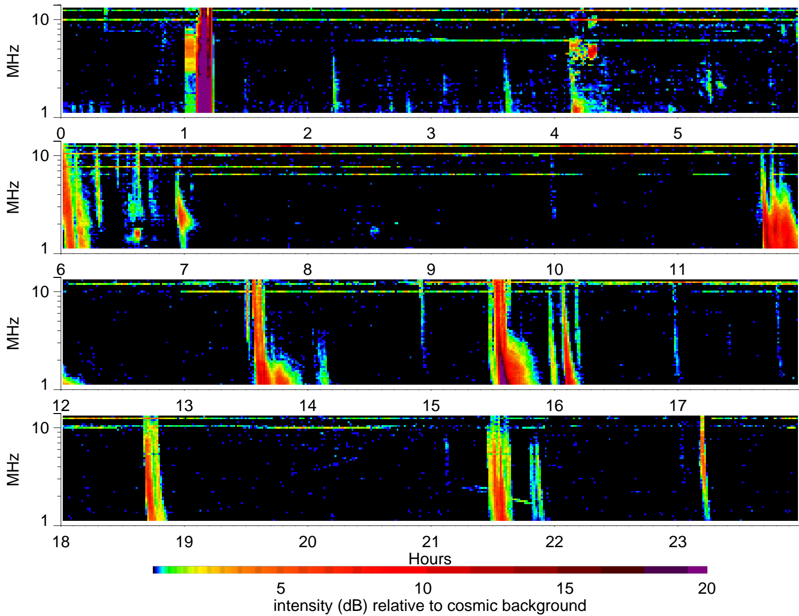
Wind Waves RAD2 receiver: 2004/7/28
