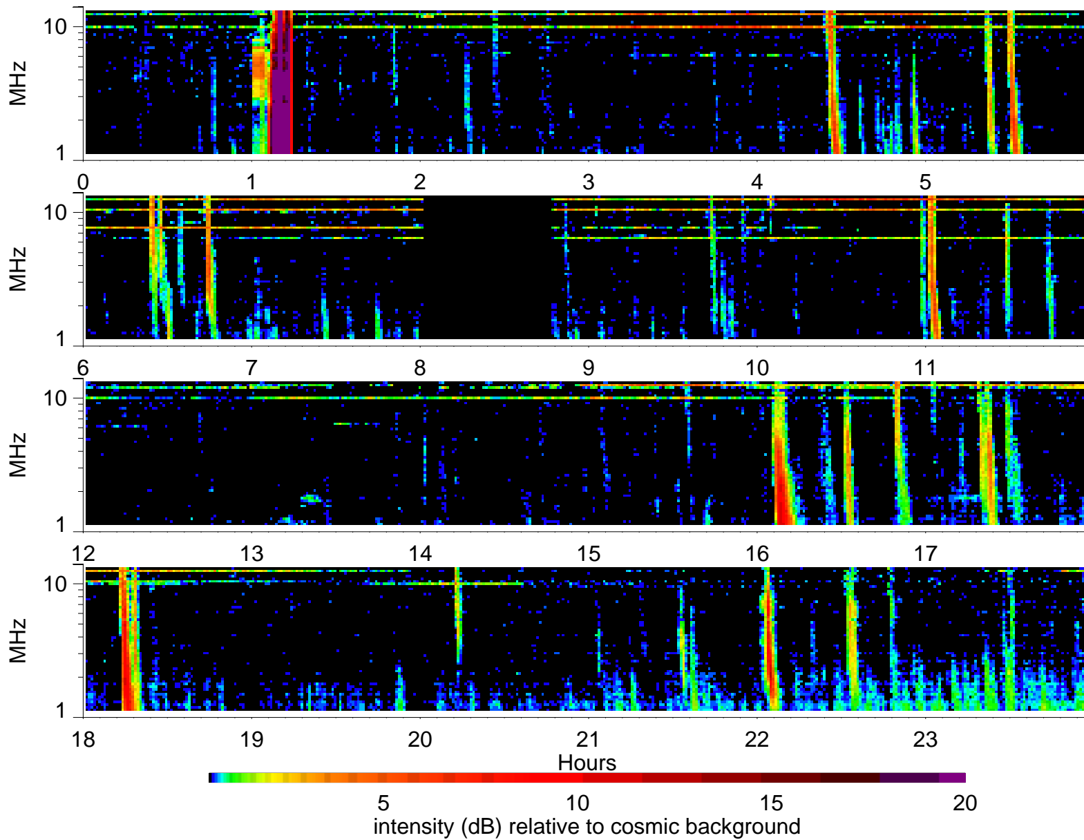
Wind Waves RAD2 receiver: 2004/7/26
