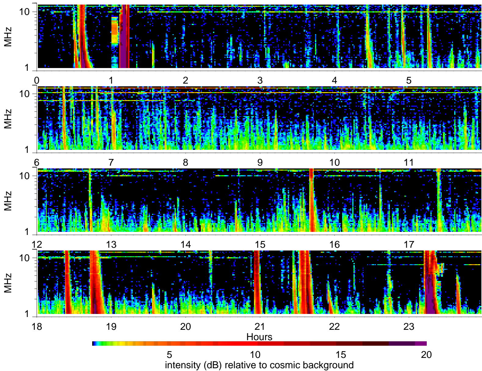
Wind Waves RAD2 receiver: 2004/7/24
