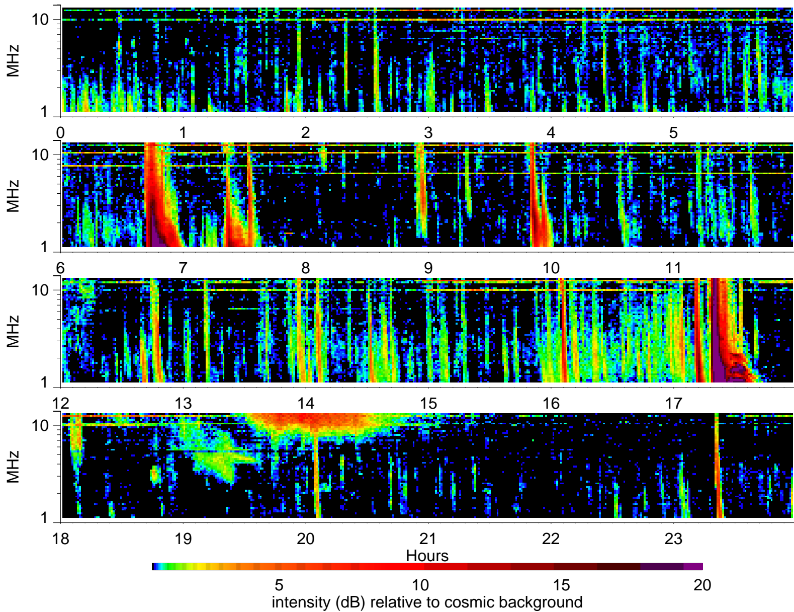
Wind Waves RAD2 receiver: 2004/7/23
