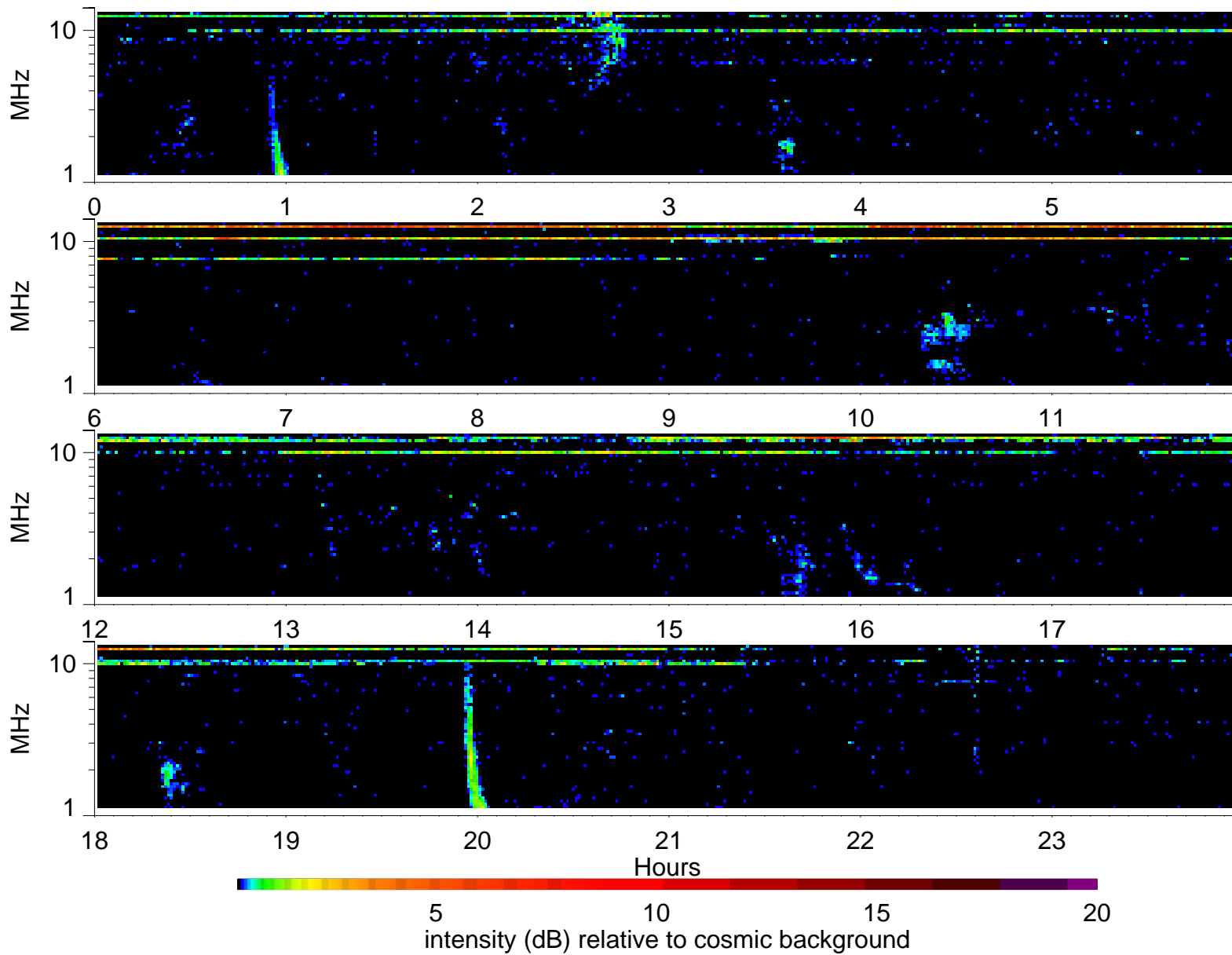
Wind Waves RAD2 receiver: 2004/7/11
