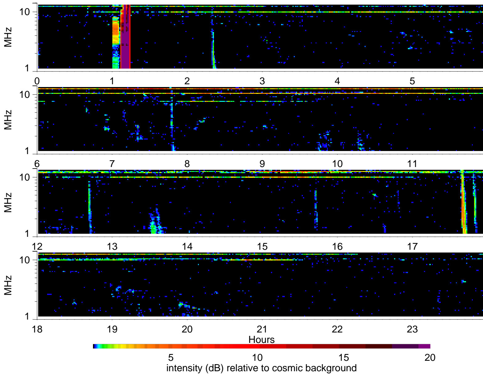
Wind Waves RAD2 receiver: 2004/7/10
