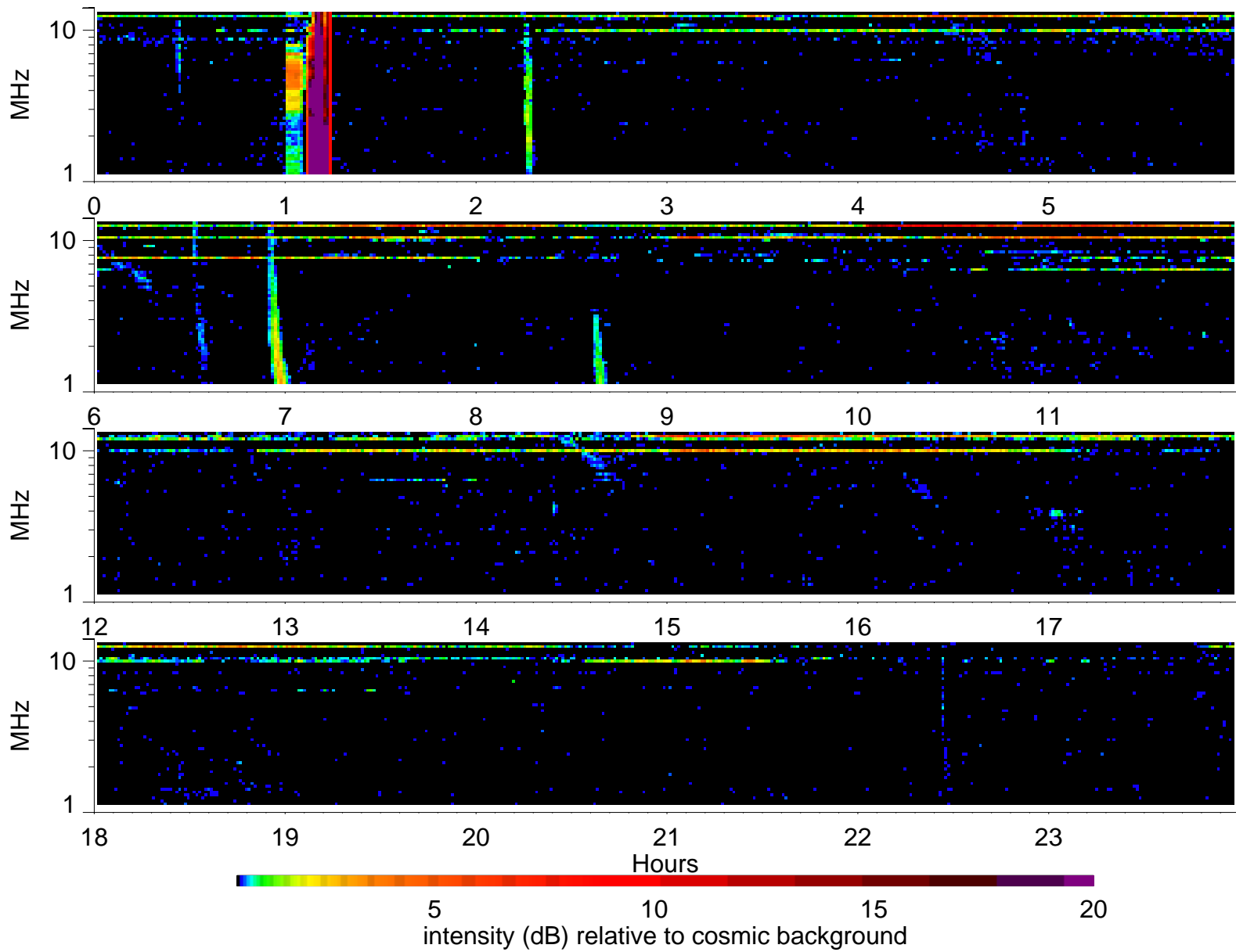
Wind Waves RAD2 receiver: 2004/7/8
