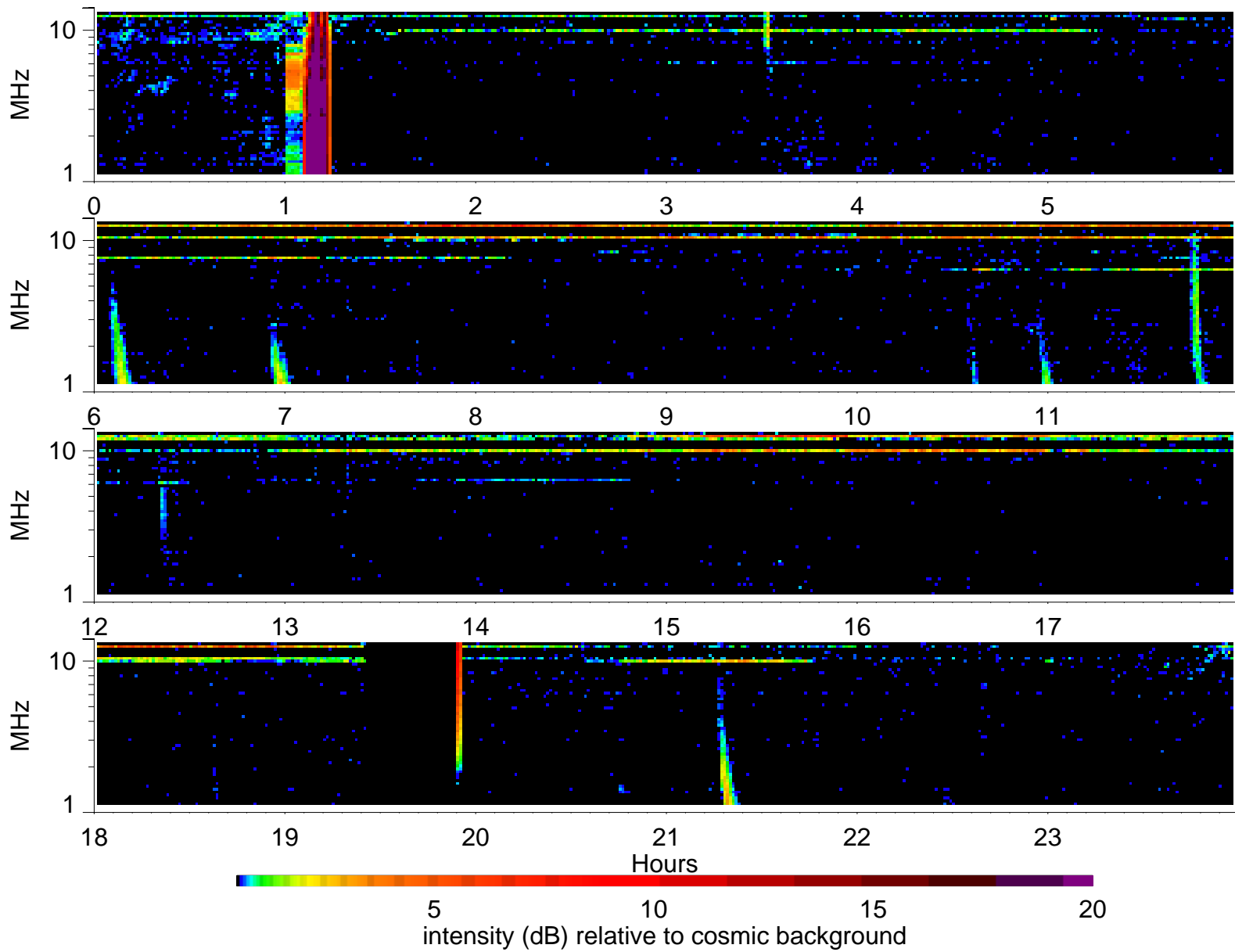
Wind Waves RAD2 receiver: 2004/7/4
