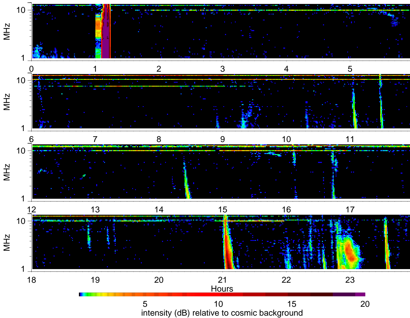
Wind Waves RAD2 receiver: 2004/6/26
