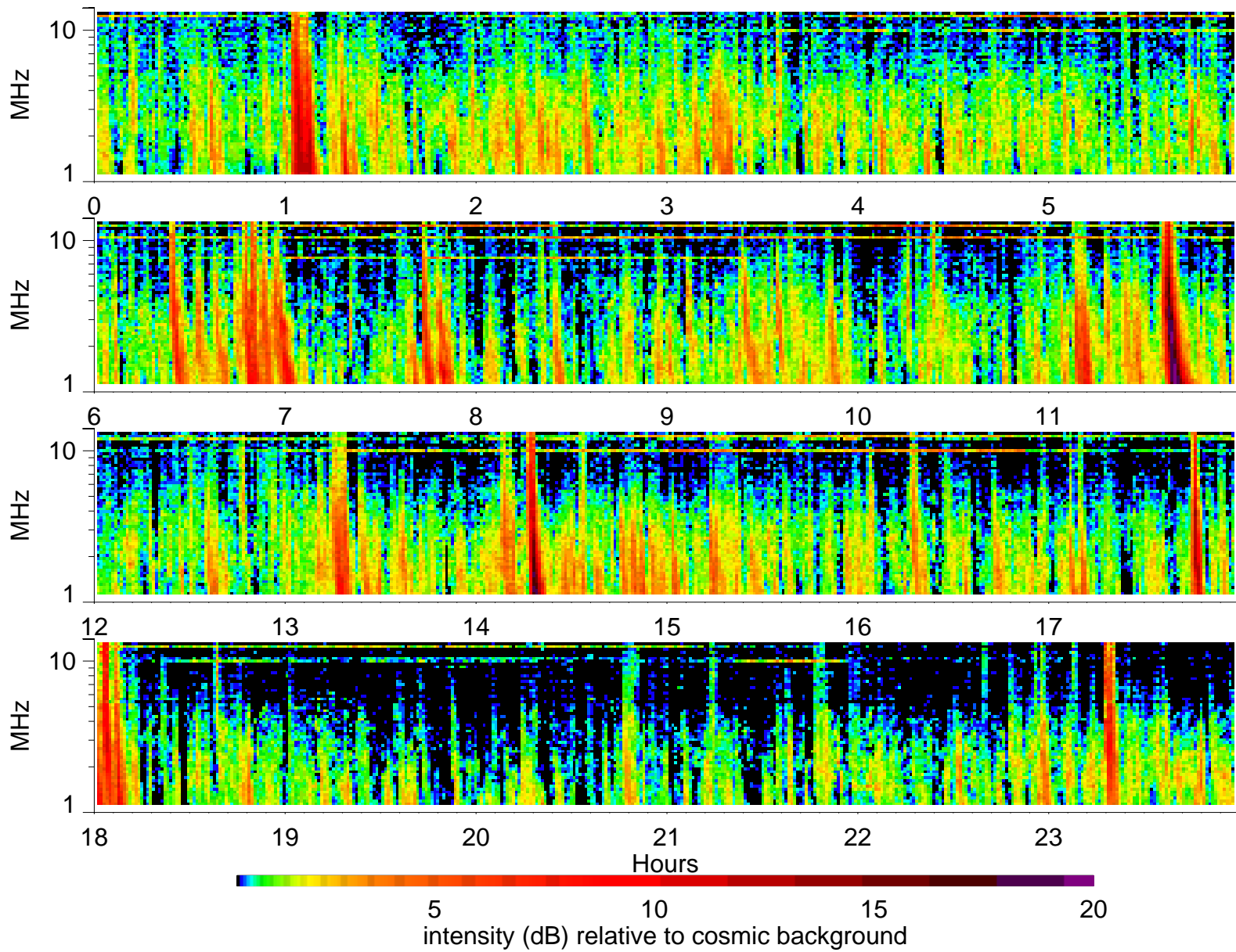
Wind Waves RAD2 receiver: 2004/6/21
