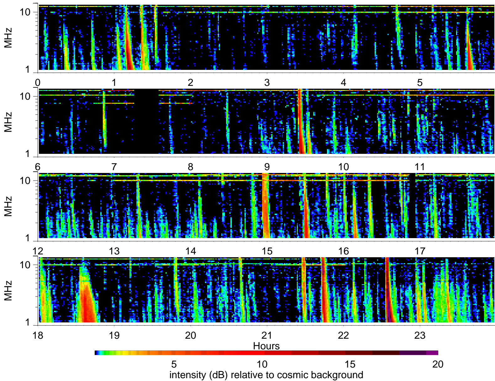
Wind Waves RAD2 receiver: 2004/6/17
