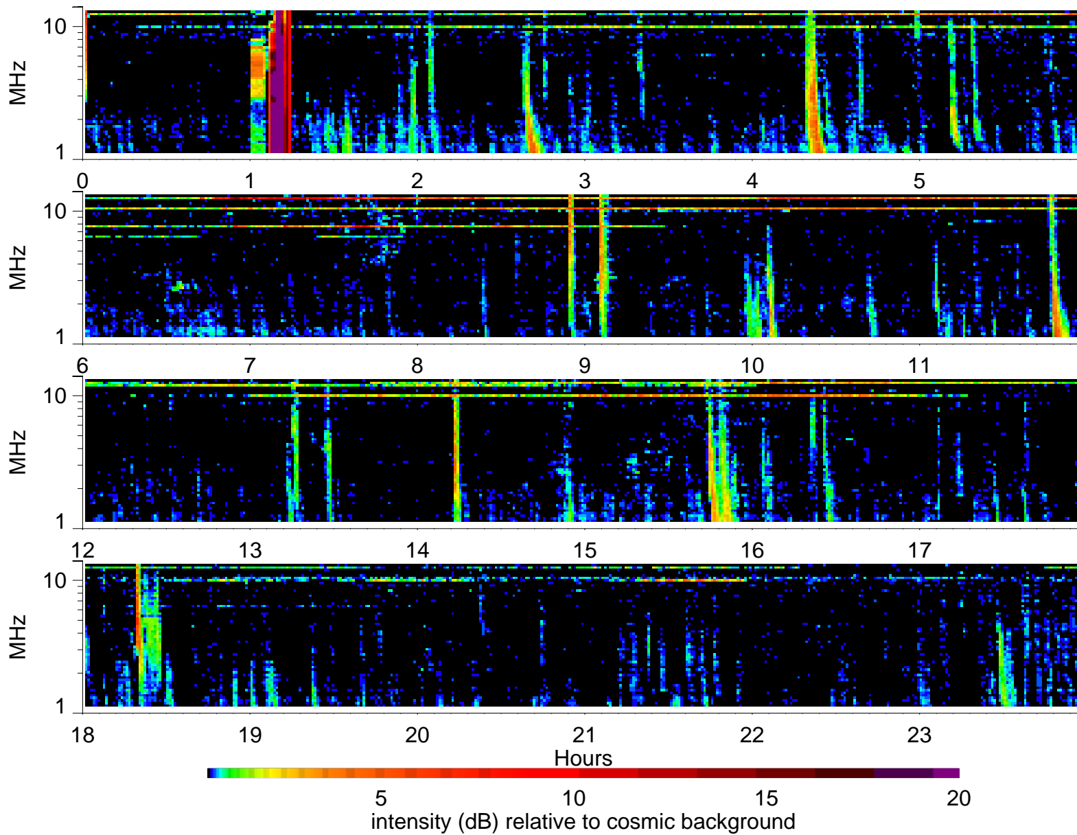
Wind Waves RAD2 receiver: 2004/6/16
