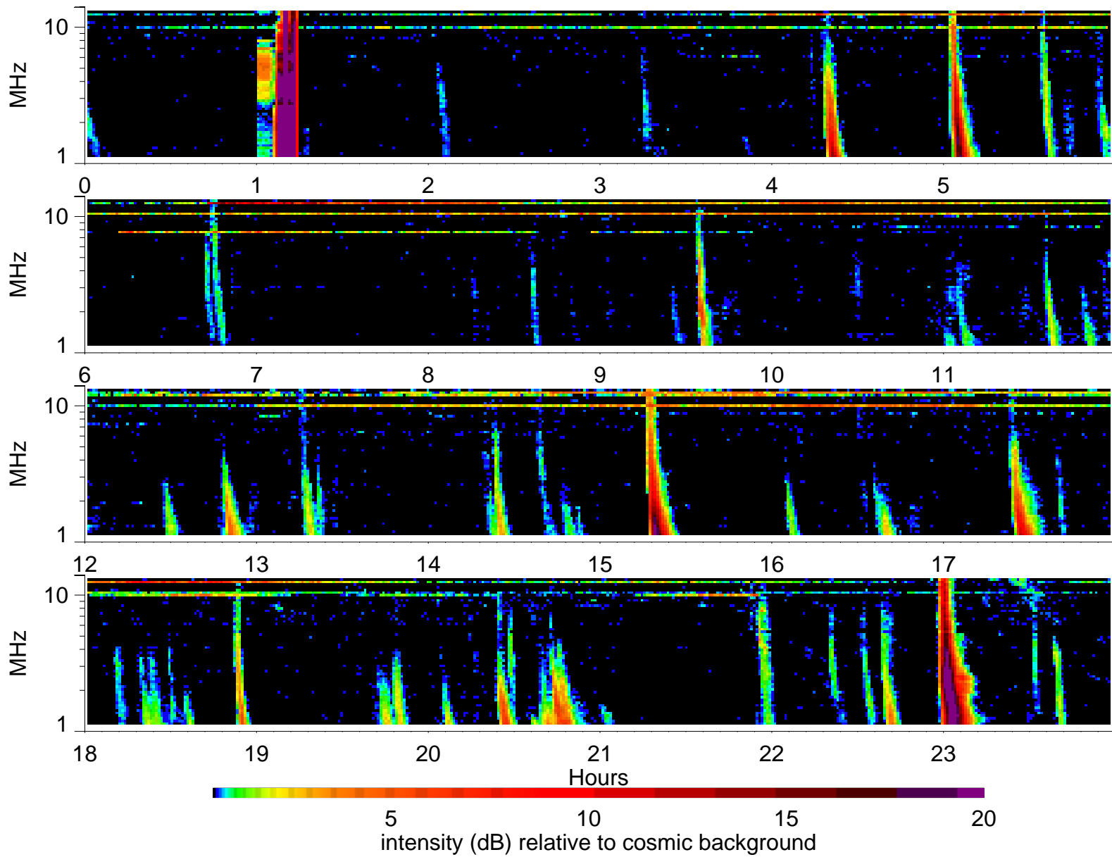
Wind Waves RAD2 receiver: 2004/6/2
