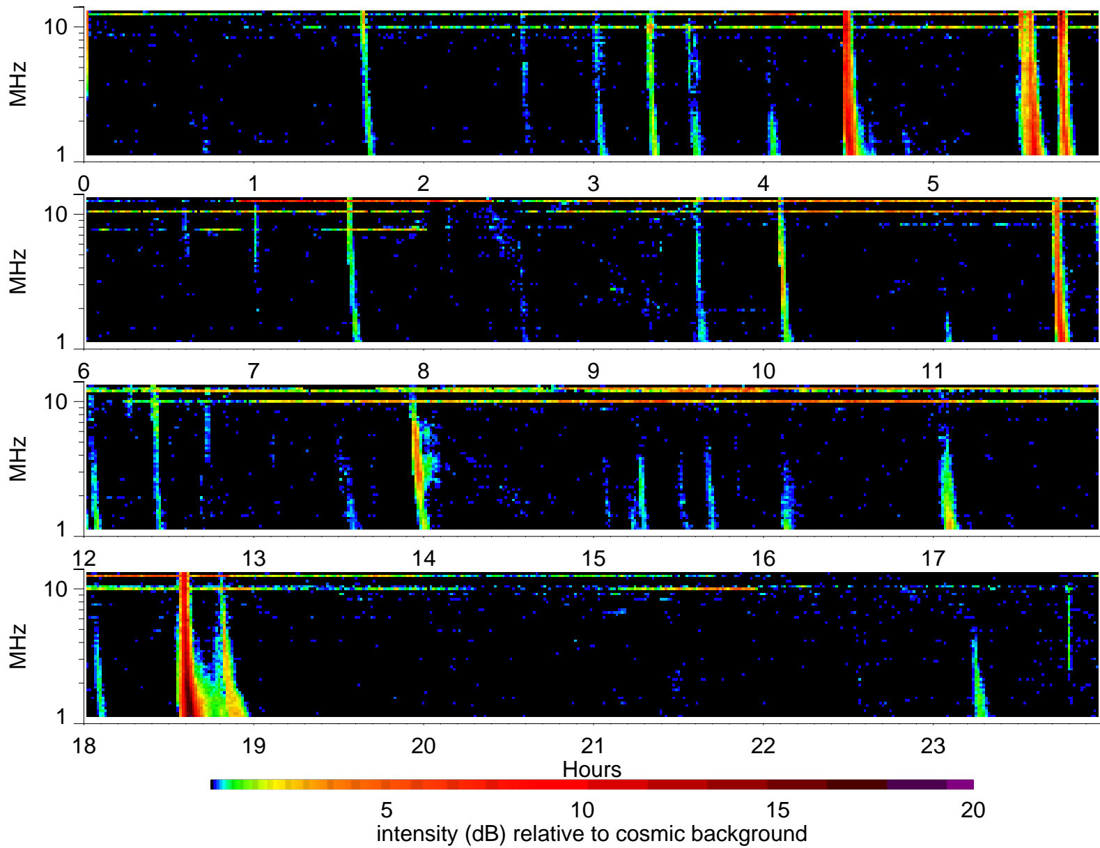
Wind Waves RAD2 receiver: 2004/6/1
