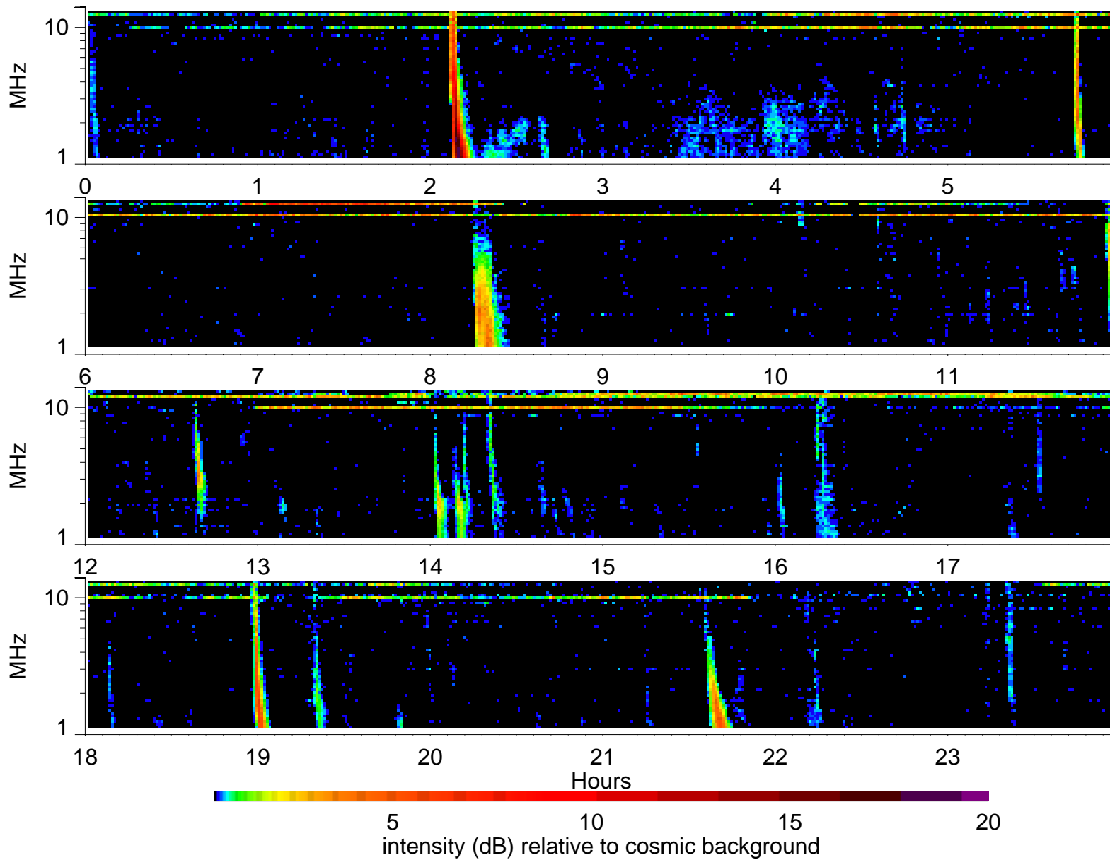
Wind Waves RAD2 receiver: 2004/5/18
