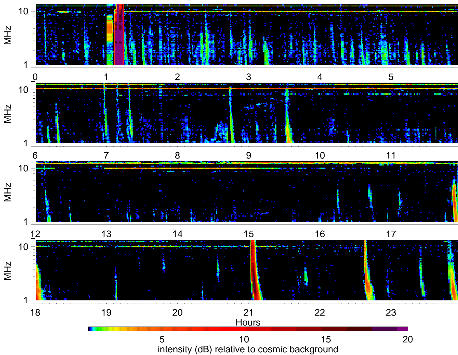
Wind Waves RAD2 receiver: 2004/5/17
