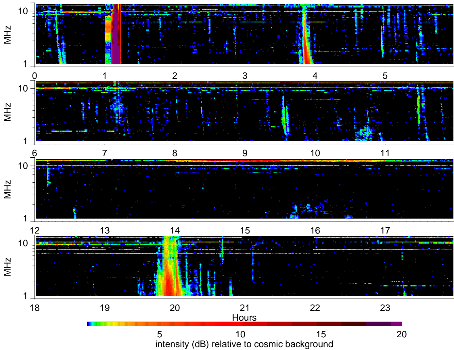
Wind Waves RAD2 receiver: 2004/5/5
