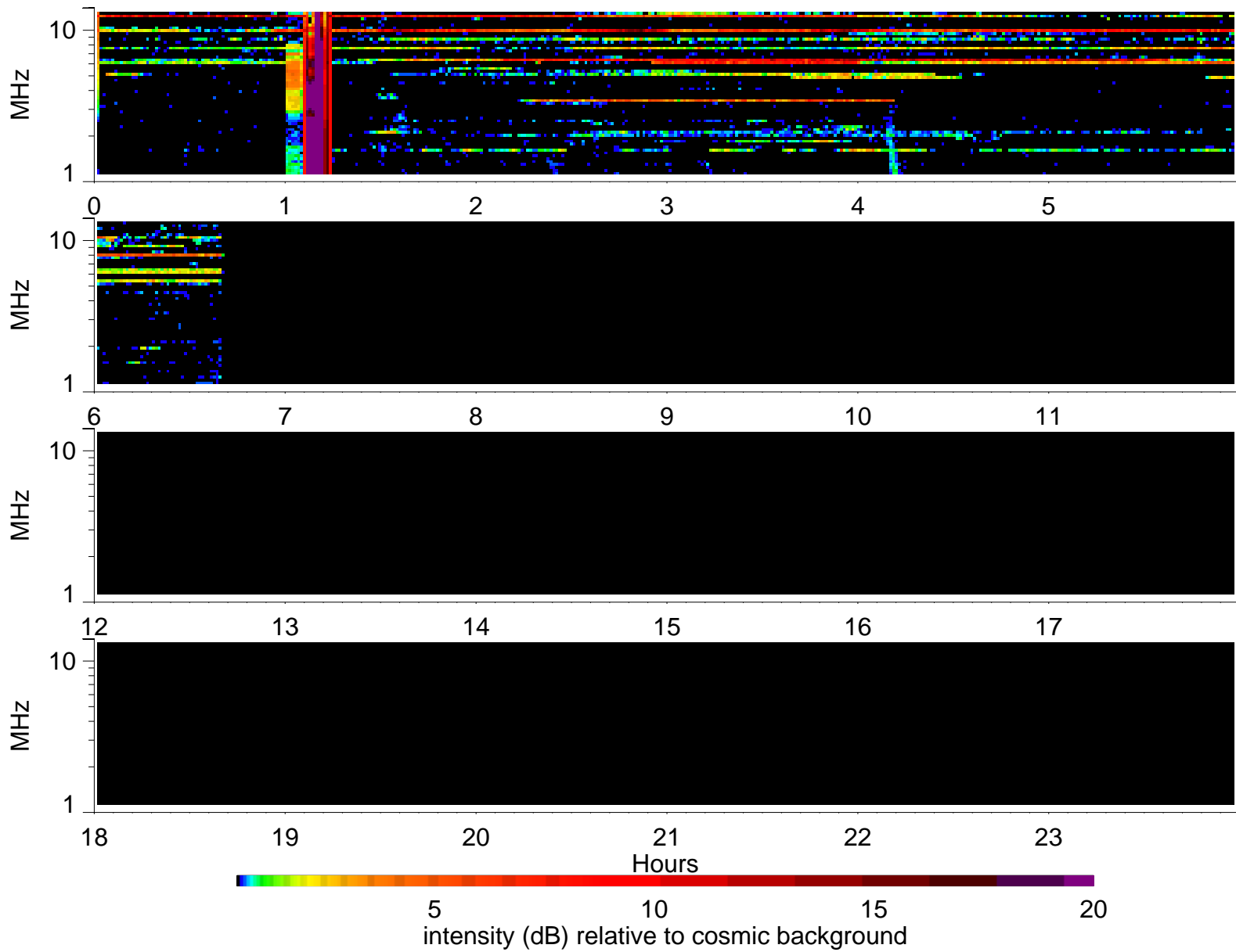
Wind Waves RAD2 receiver: 2004/5/1
