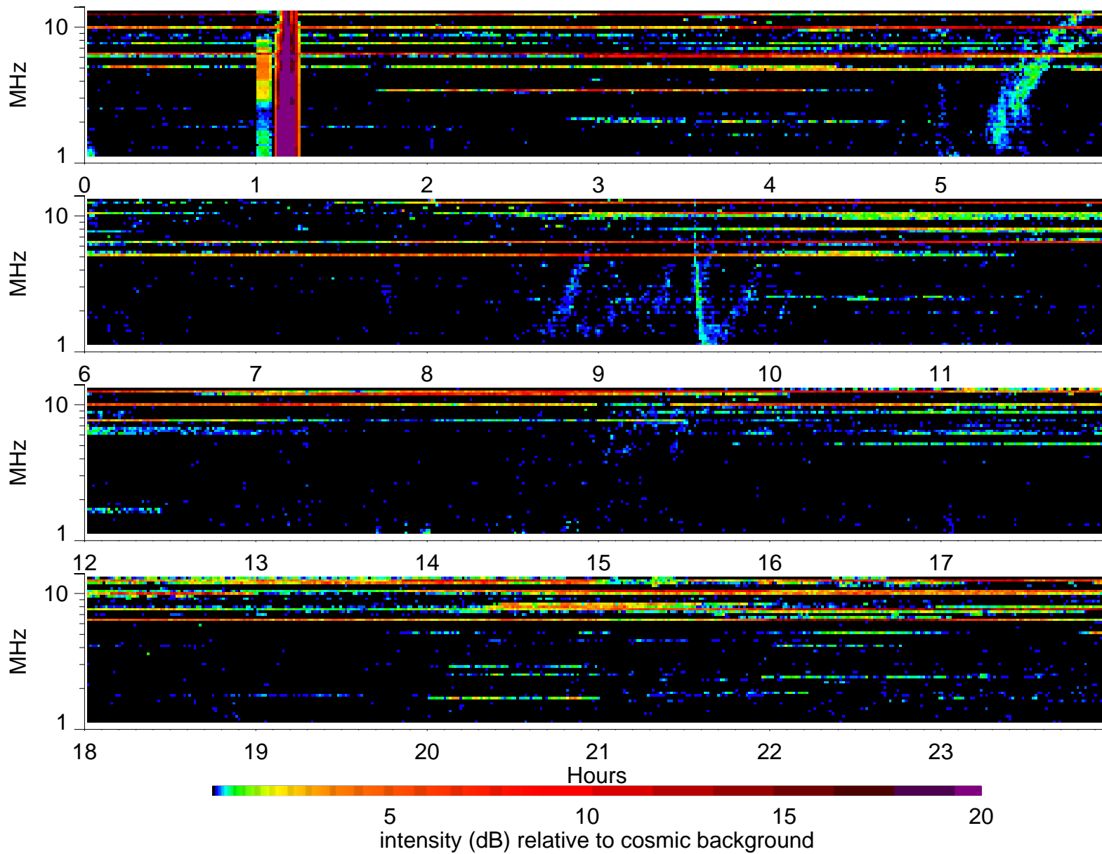
Wind Waves RAD2 receiver: 2004/4/29
