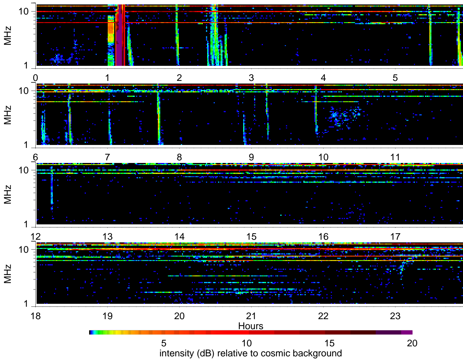
Wind Waves RAD2 receiver: 2004/4/23
