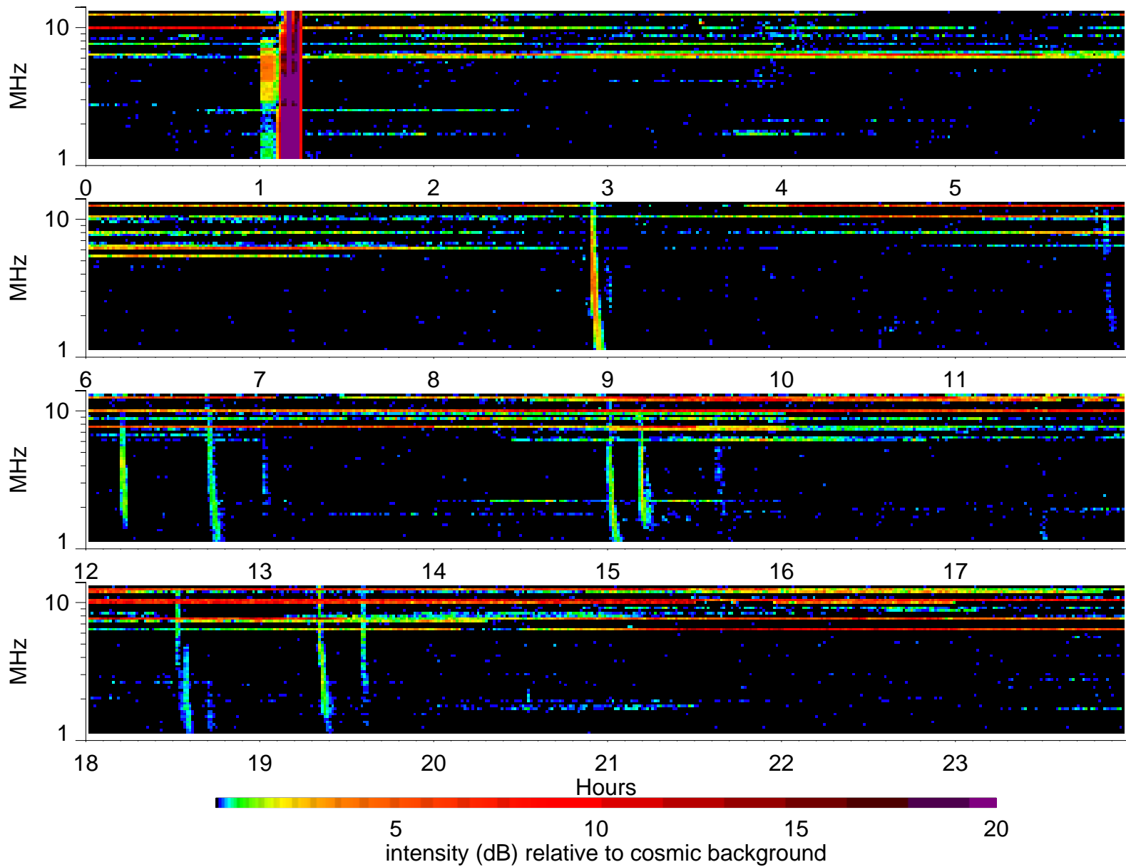
Wind Waves RAD2 receiver: 2004/4/17
