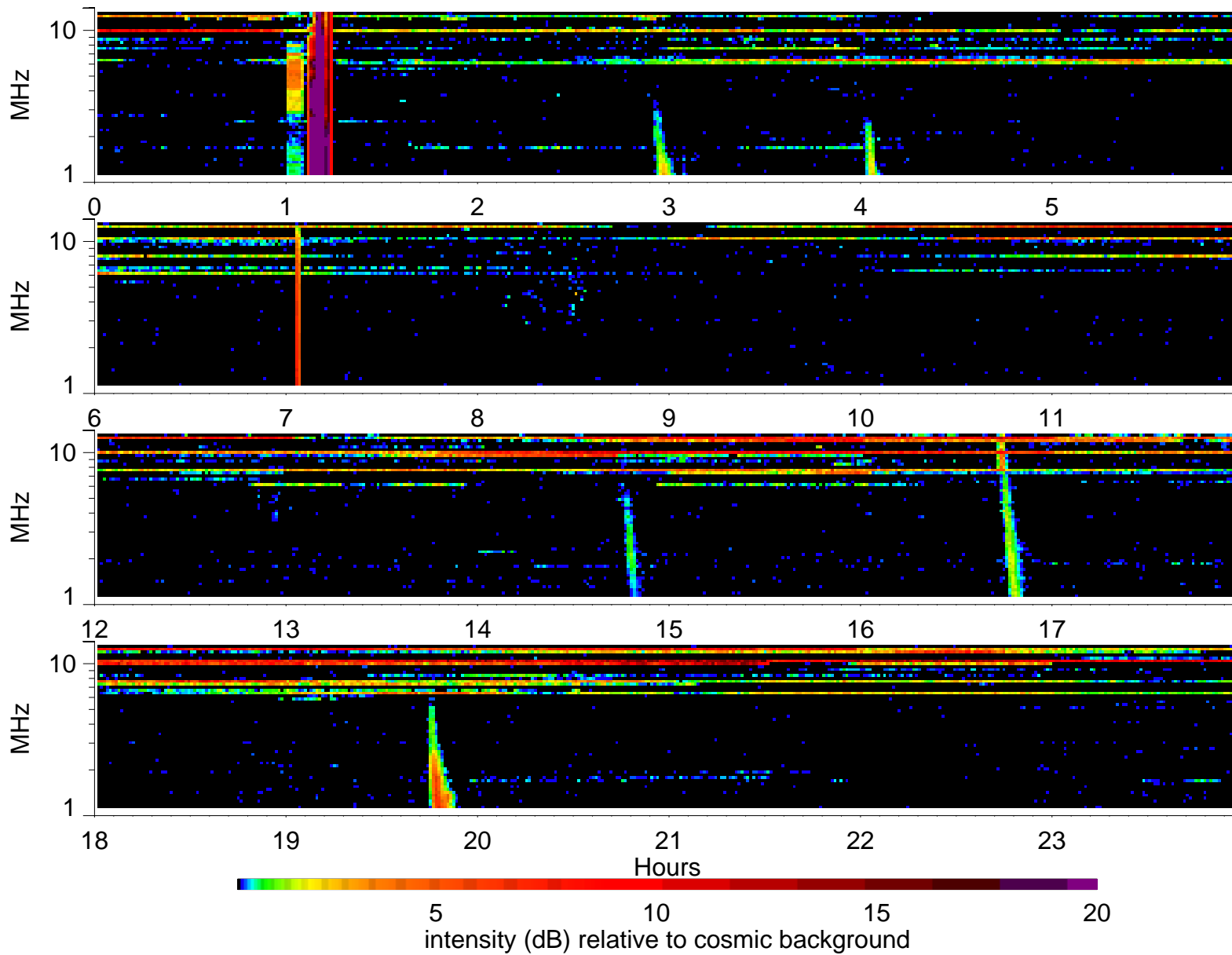
Wind Waves RAD2 receiver: 2004/4/15
