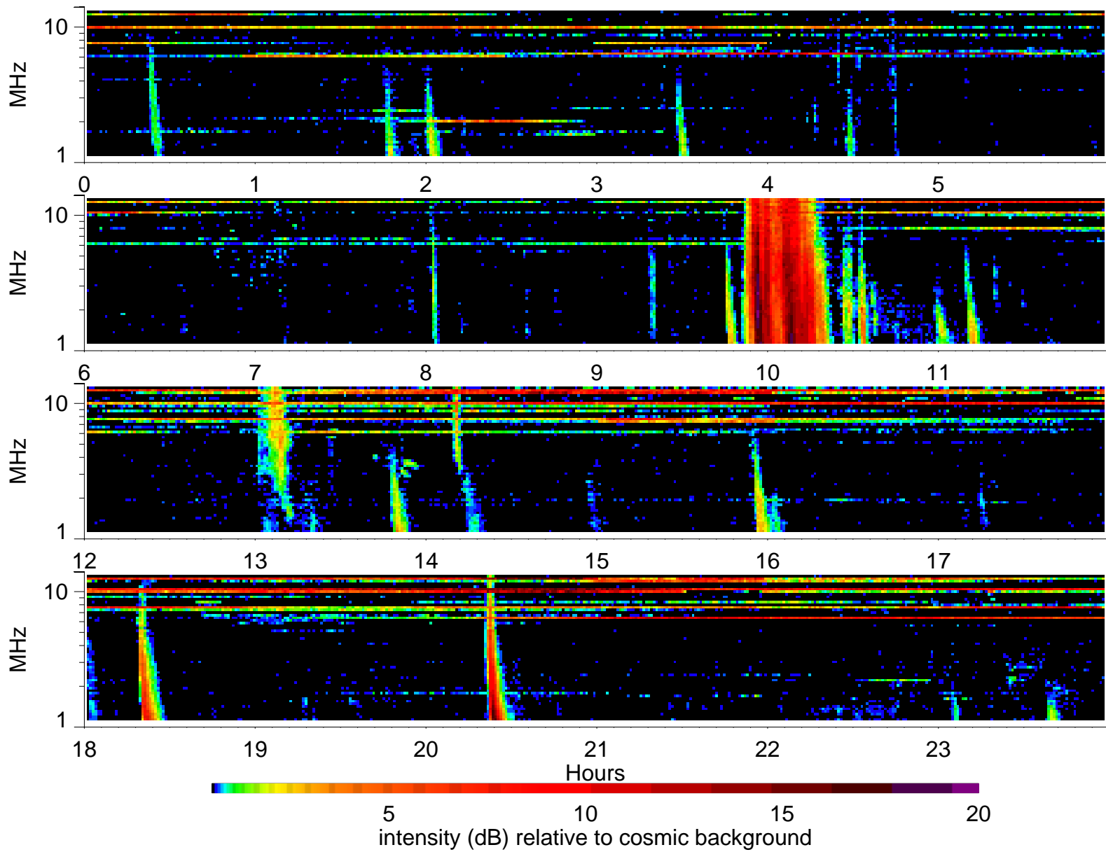
Wind Waves RAD2 receiver: 2004/4/8
