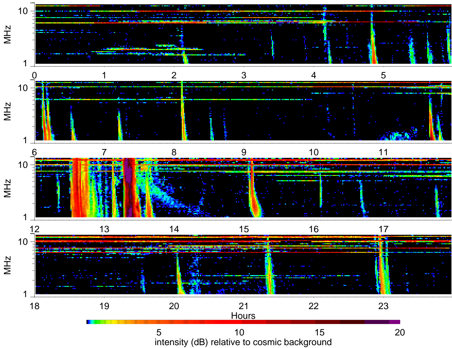
Wind Waves RAD2 receiver: 2004/4/6
