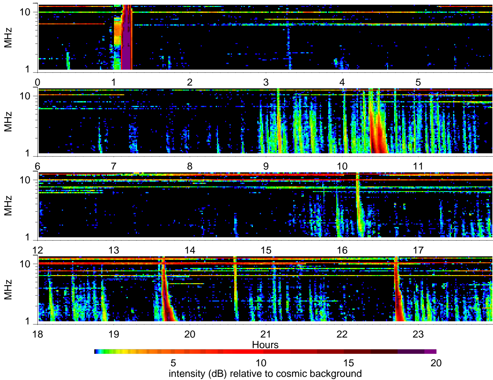
Wind Waves RAD2 receiver: 2004/4/3
