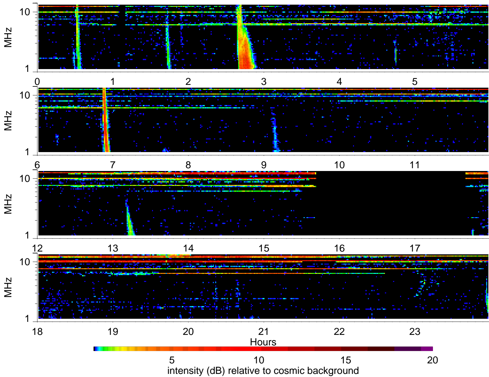
Wind Waves RAD2 receiver: 2004/4/2
