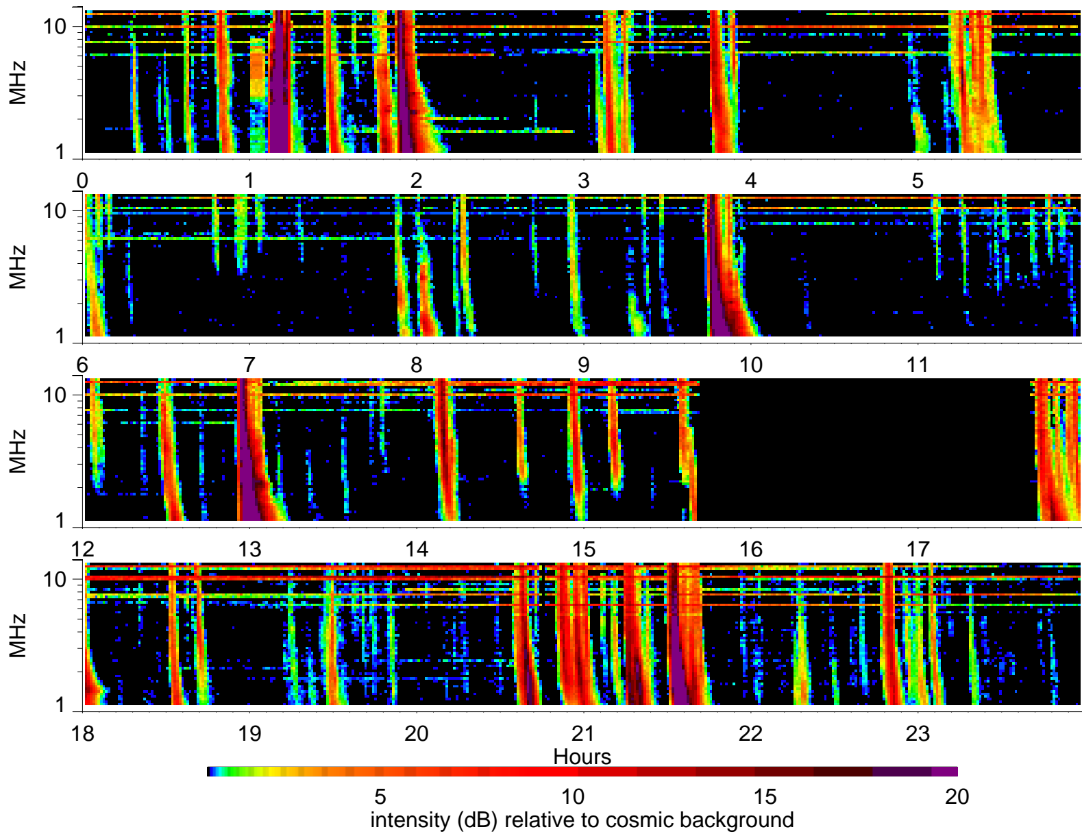
Wind Waves RAD2 receiver: 2004/3/30
