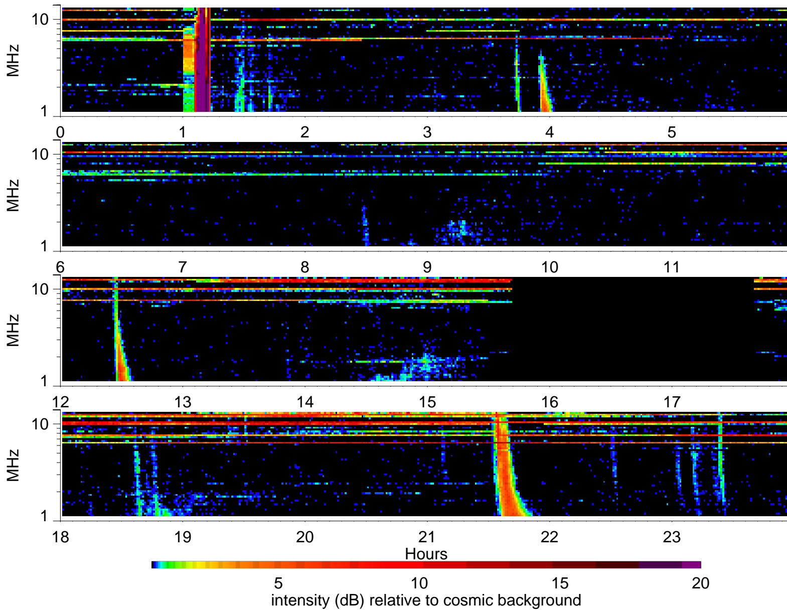
Wind Waves RAD2 receiver: 2004/3/28
