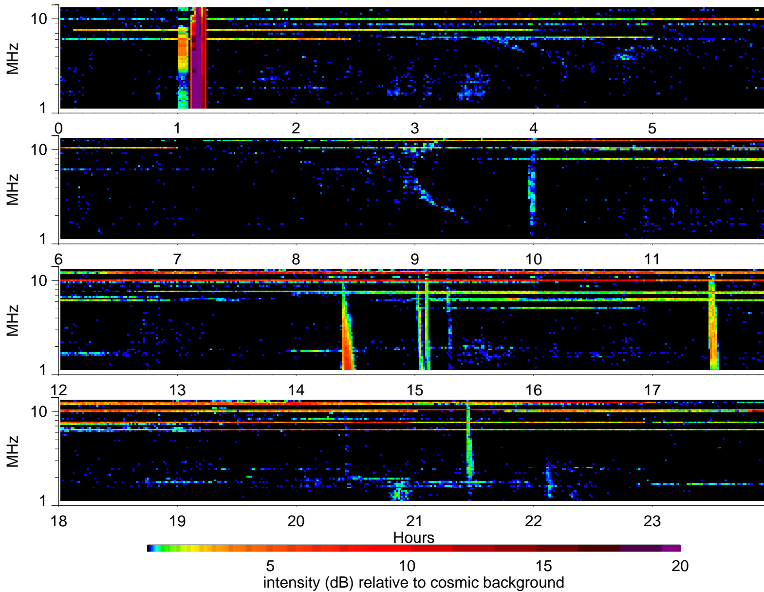
Wind Waves RAD2 receiver: 2004/3/24
