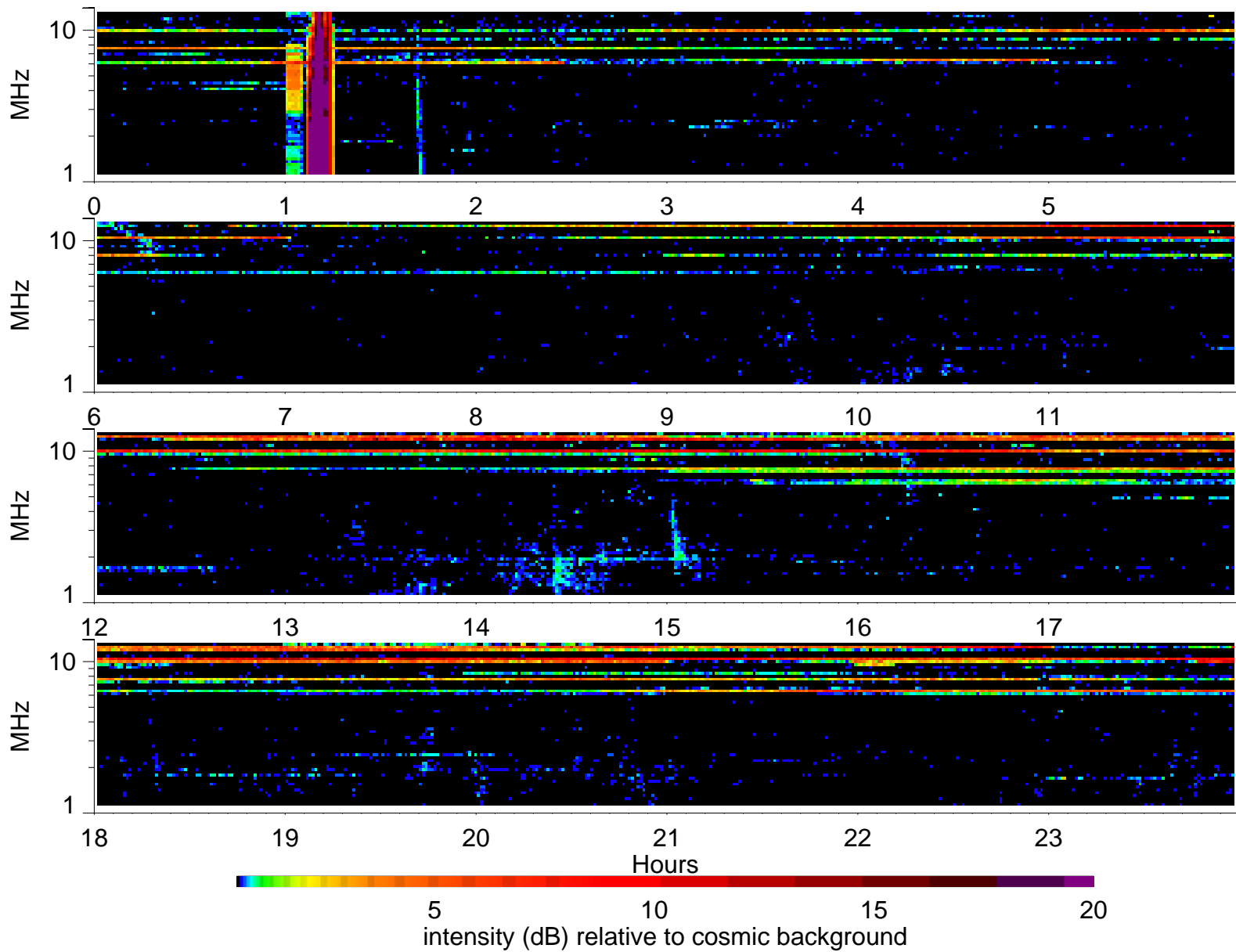
Wind Waves RAD2 receiver: 2004/3/22
